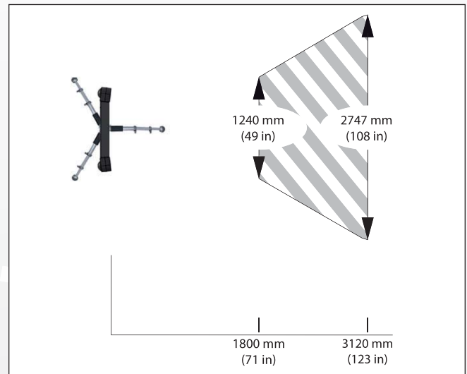
2. TOP VIEW
